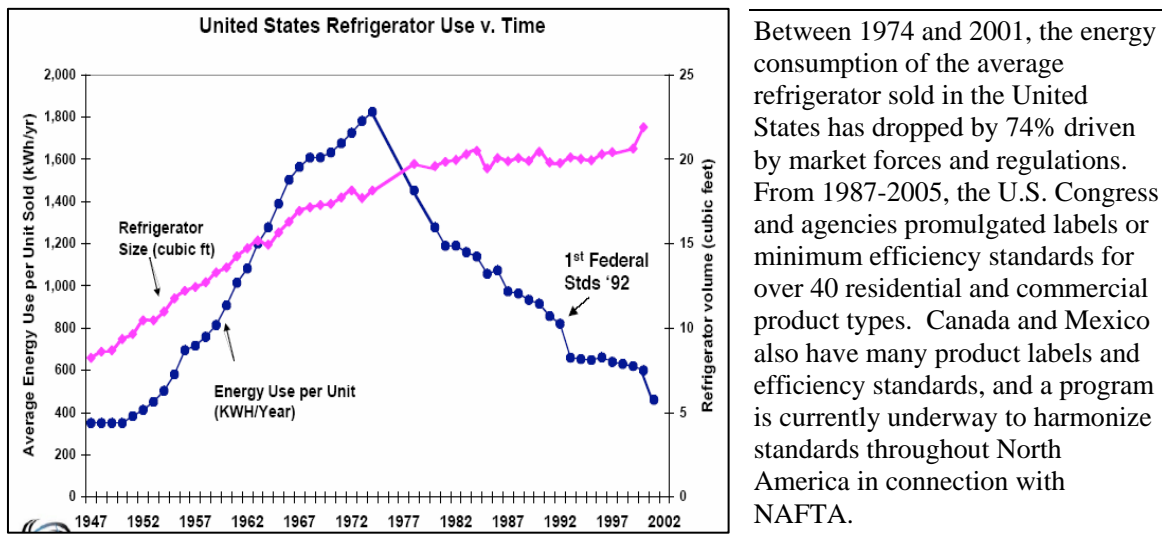
Figure 10: US Historical Refrigerator Electricity Consumption
