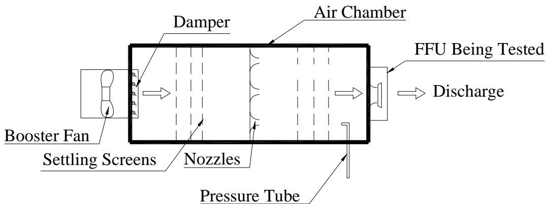
Figure 1 Laboratory measurement layout
