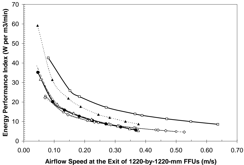
Figure 5 FFUs' Energy Performance Index at 125-Pa Pressure Rise
