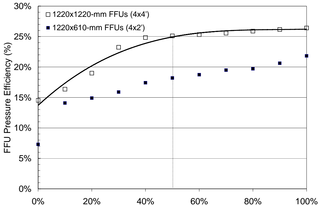
Figure 4 Comparison of FFUs' Pressure Efficiency at 125-Pa Pressure Rise
