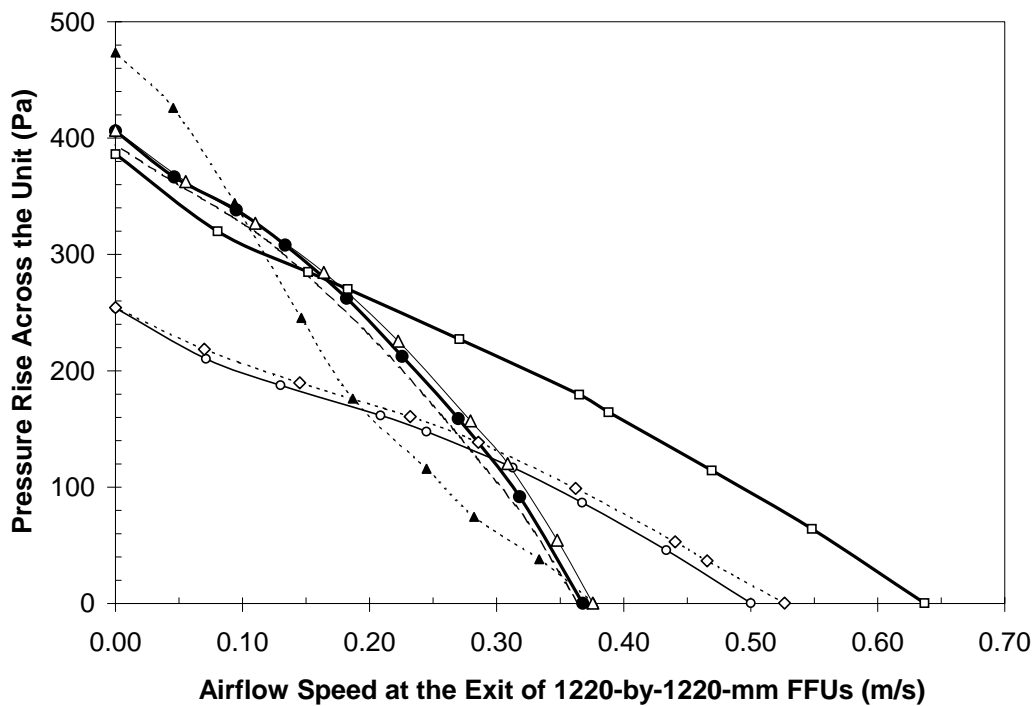
Figure 2 Pressure rise across the unit and airflow speed at FFU exit
